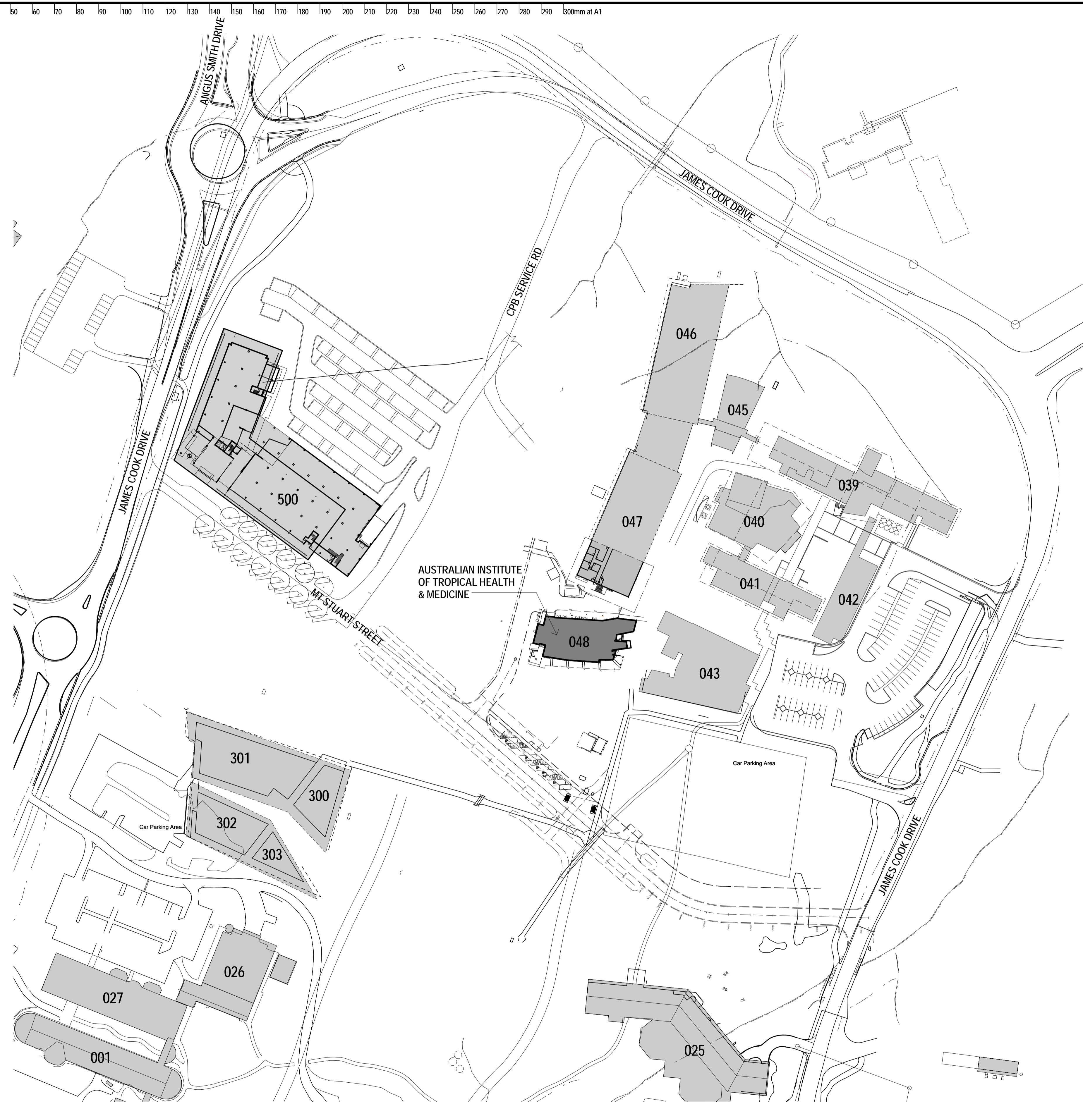
1 LOCATION PLAN 1:1000
