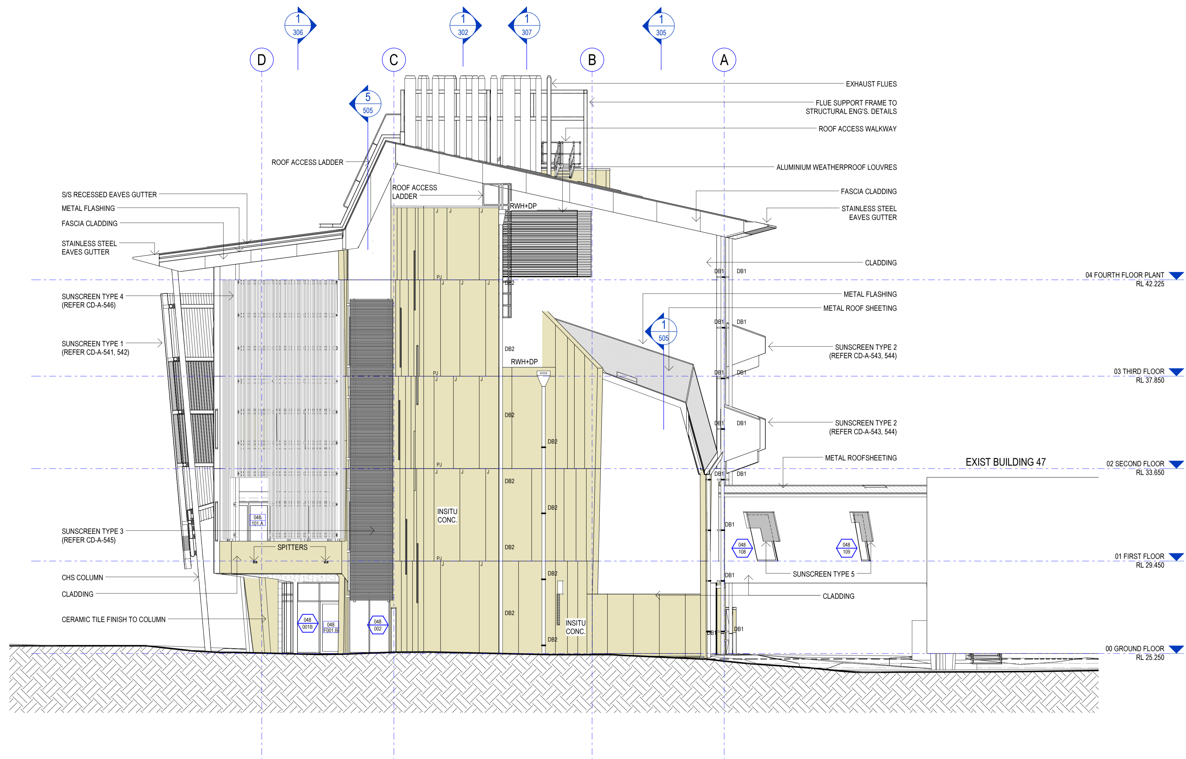
1 EAST ELEVATION 1:100
