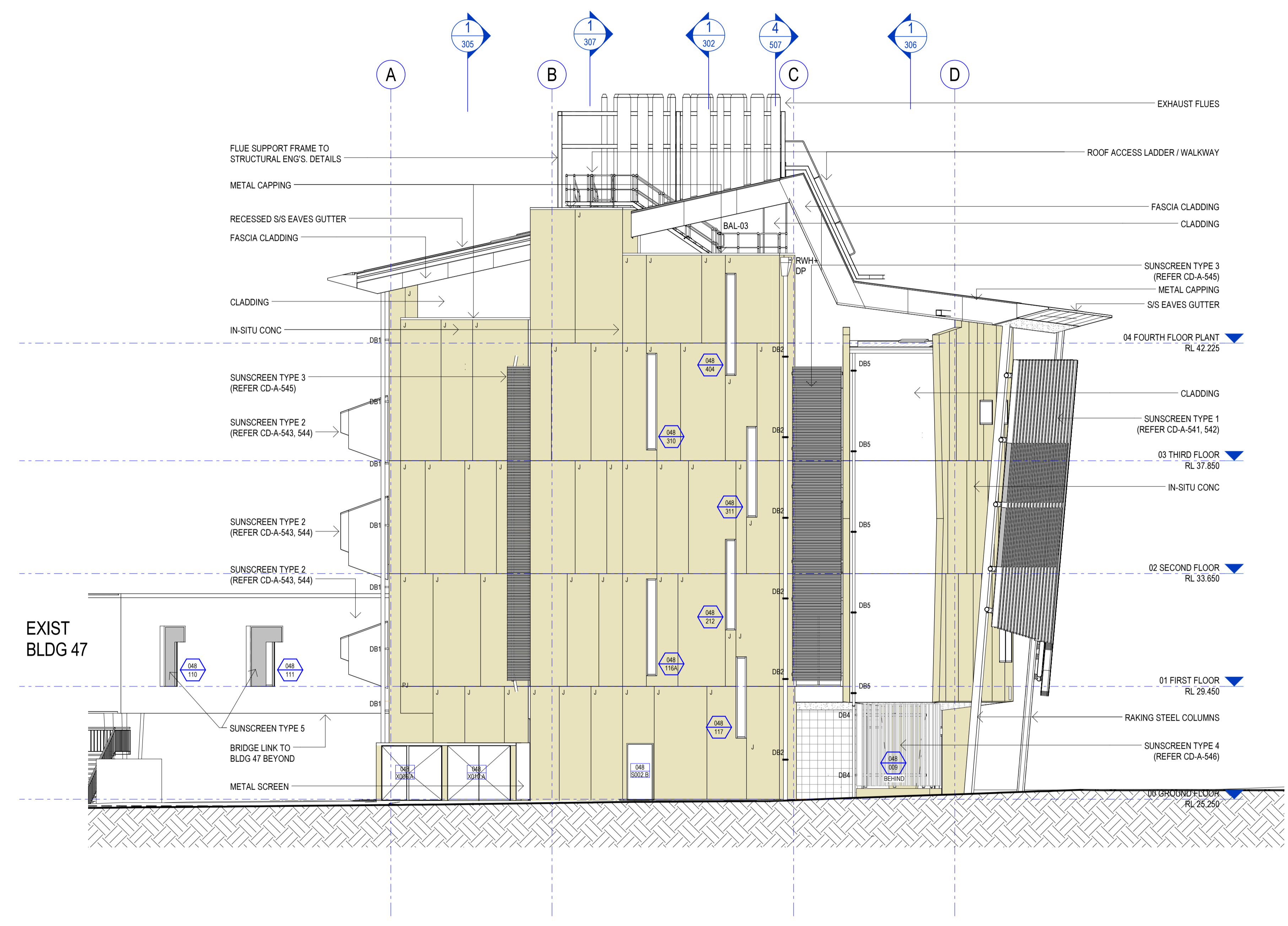
1 WEST ELEVATION 1:100
